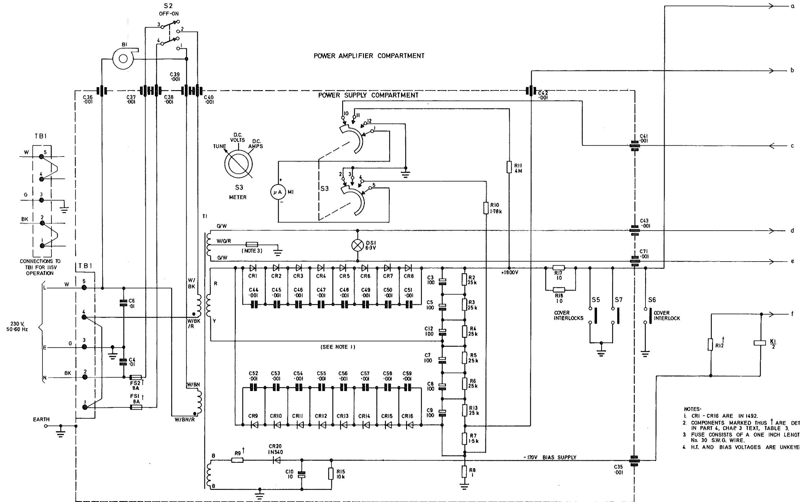
R.F linear amplifier 30L-1 - circuit
